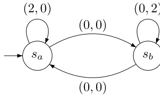
Fig. 3. A multi-mean-payoff game where infinite memory is necessary to win (Lemma 7).
