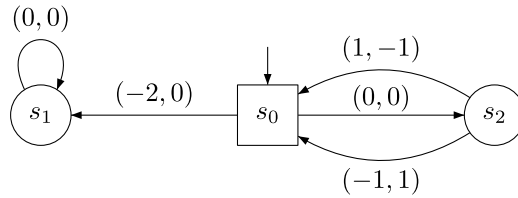
Fig. 1. player 1 (round states) wins with initial credit (2, 0) when player 2 (square states) can use memoryless strategies, but not when player 2 can use arbitrary strategies.
