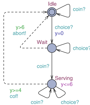
Fig. 2. Non-robust specification of a coffee machine.
