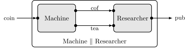
Fig. 10. Diagram for the parallel composition of a coffee machine and a researcher.
