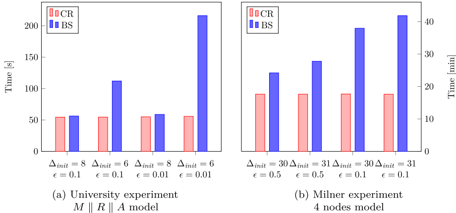
Fig. 11. Comparisons of the performances between the two methods Counter strategy Refinement (CR) and Binary Search (BS).
