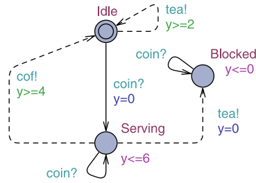
Fig. 5. Consistent specification with error states.
