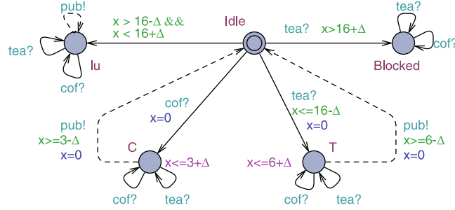
Fig. 7. \Delta -perturbation of the researcher implementation.
