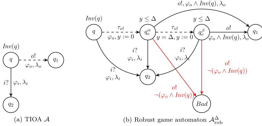
Fig. 8. Illustration of the construction of the robust game automaton \mathcal{A}_{\text{rob}}^{\Delta} , from an automaton \mathcal{A} , with one location q and incident edges e = (q, o!, \varphi_o, \lambda_o, q_1) and (q, i?, \varphi_i, \lambda_i, q_2) .
