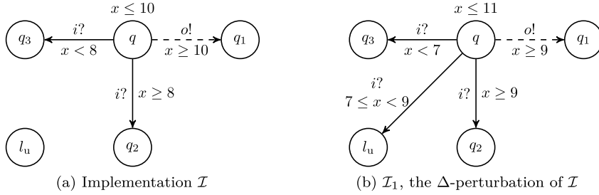
Fig. 6. Illustration of the \Delta -perturbation of an implementation \mathcal{I} by \Delta = 1 .
