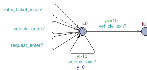
Fig. 13. Assumption on the environment of the parking controller.
