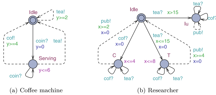
Fig. 1. Timed specifications with timed I/O automata.
