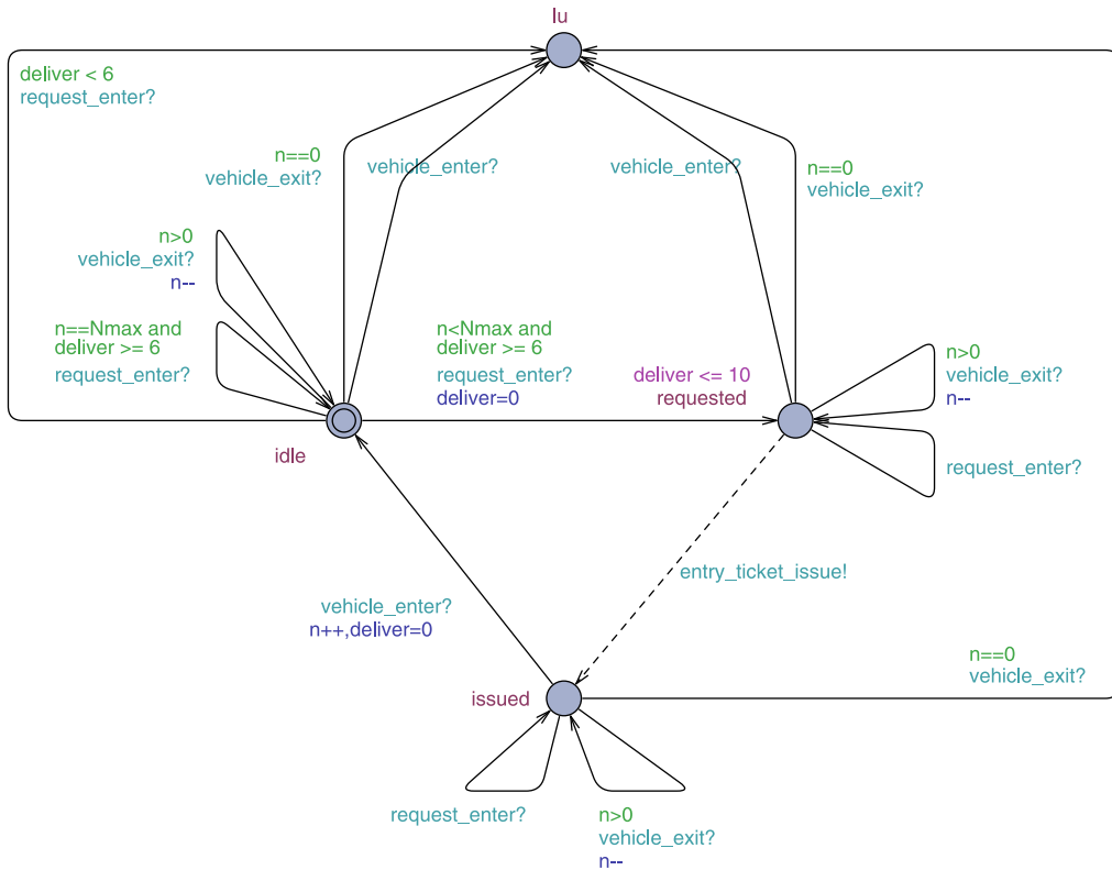
Fig. 12. Specification of the parking controller.
