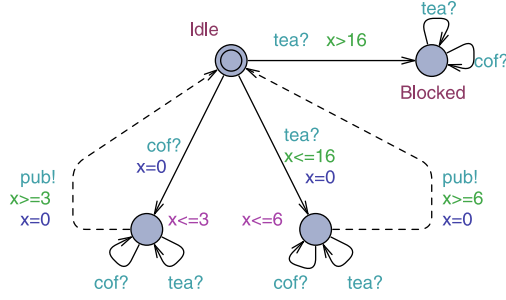
Fig. 3. Implementation for a researcher.
