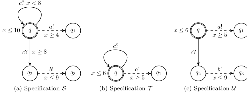
Fig. 4. Refinement between specifications: \mathcal{T} \leq \mathcal{S} , but \mathcal{U} \not\leq \mathcal{S} .
