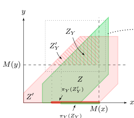
Fig. 3. Two-dimensional zones Z and Z' , and sub-zones Z_Y and Z'_Y for Y = \{x\} .
